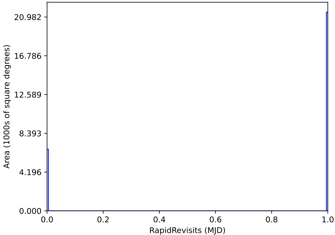
too_elab_r128_d3_ugrizy_v3.4_10yrs : RapidRevisits
