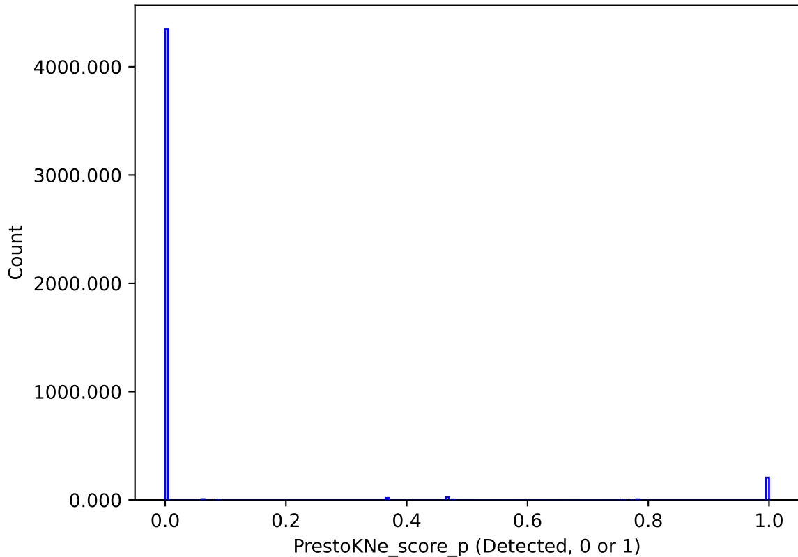
too_elab_r128_d3_ugrizy_v3.4_10yrs : PrestoKNe_score_p
