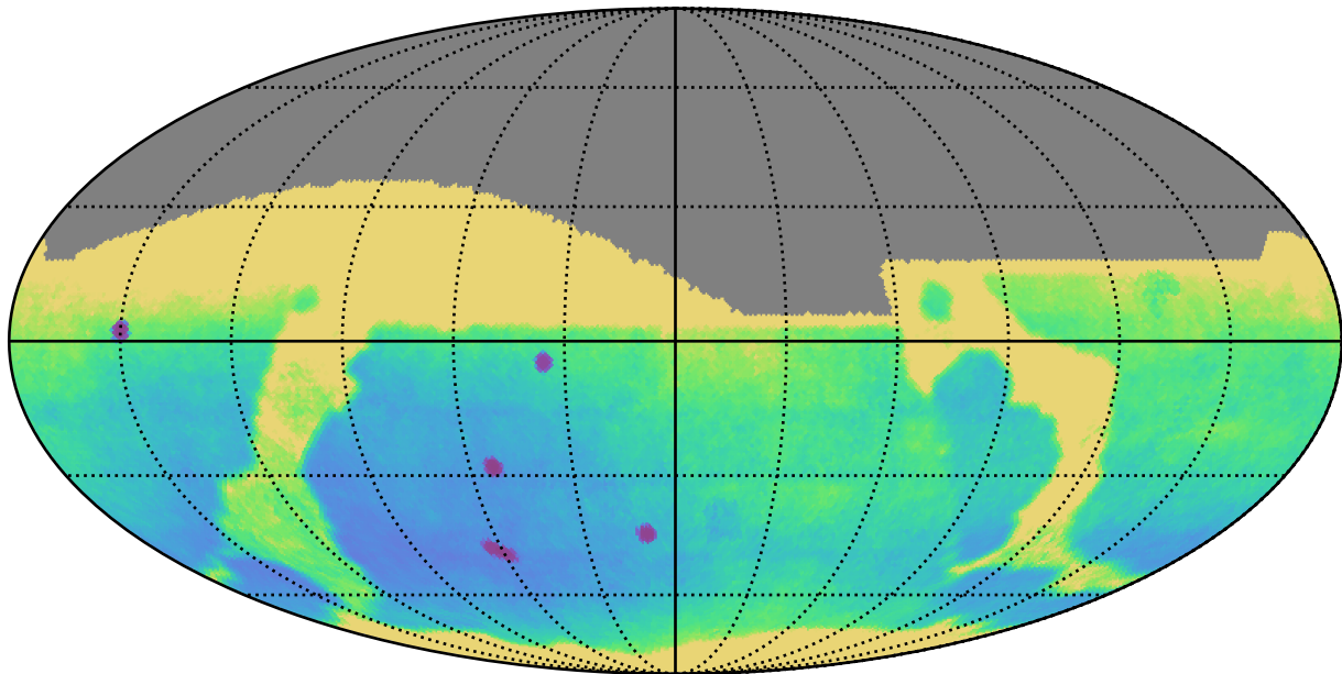
too_elab_r128_d3_ugrizy_v3.4_10yrs : Parallax Uncert @ 24.0
