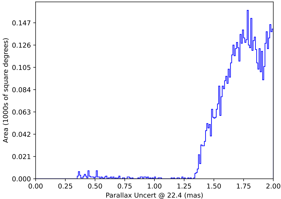
too_elab_r128_d3_ugrizy_v3.4_10yrs : Parallax Uncert @ 22.4
