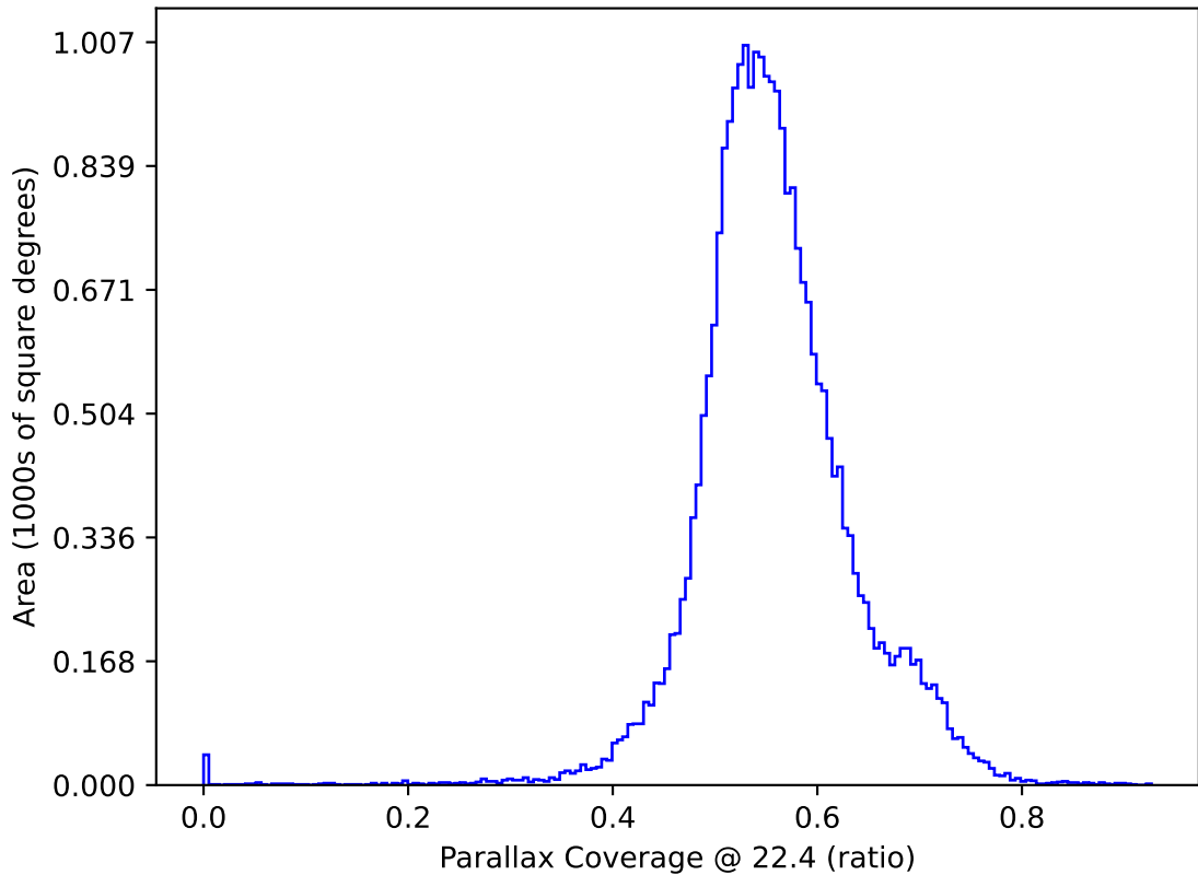
too_elab_r128_d3_ugrizy_v3.4_10yrs : Parallax Coverage @ 22.4
