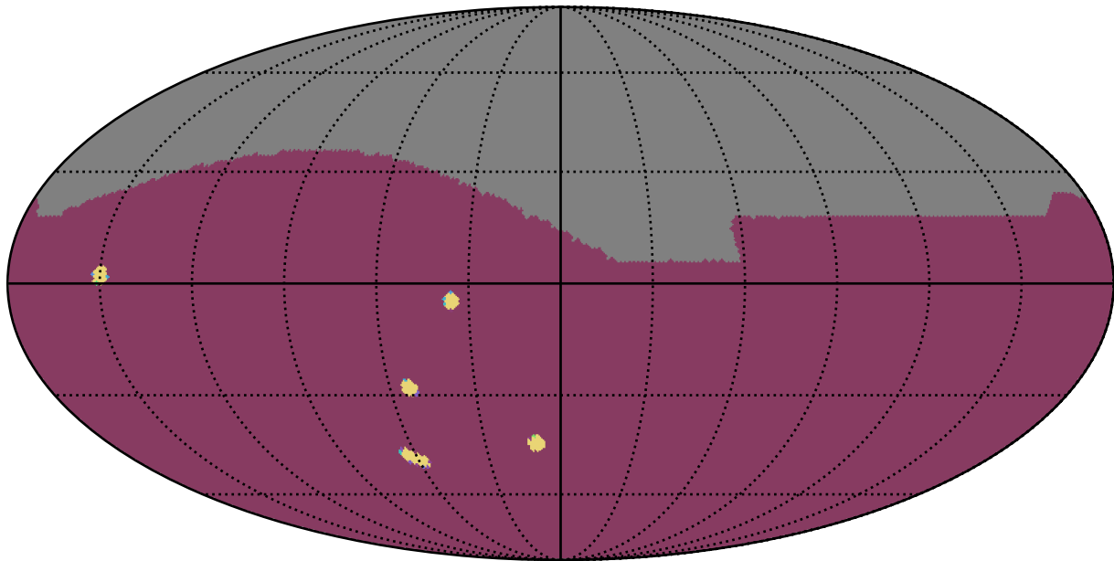
too_elab_r128_d3_ugrizy_v3.4_10yrs : NumberOfQuickRevisits
