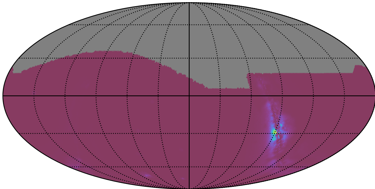
too_elab_r128_d3_ugrizy_v3.4_10yrs : NlcPoints
