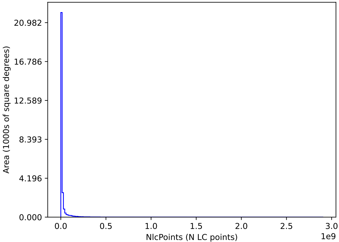
too_elab_r128_d3_ugrizy_v3.4_10yrs : NlcPoints
