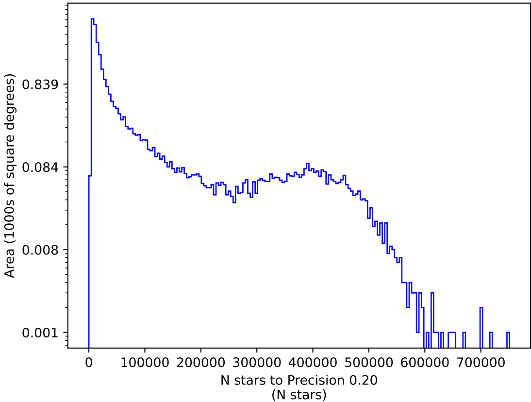
too_elab_r128_d3_ugrizy_v3.4_10yrs r: N stars to Precision 0.20
