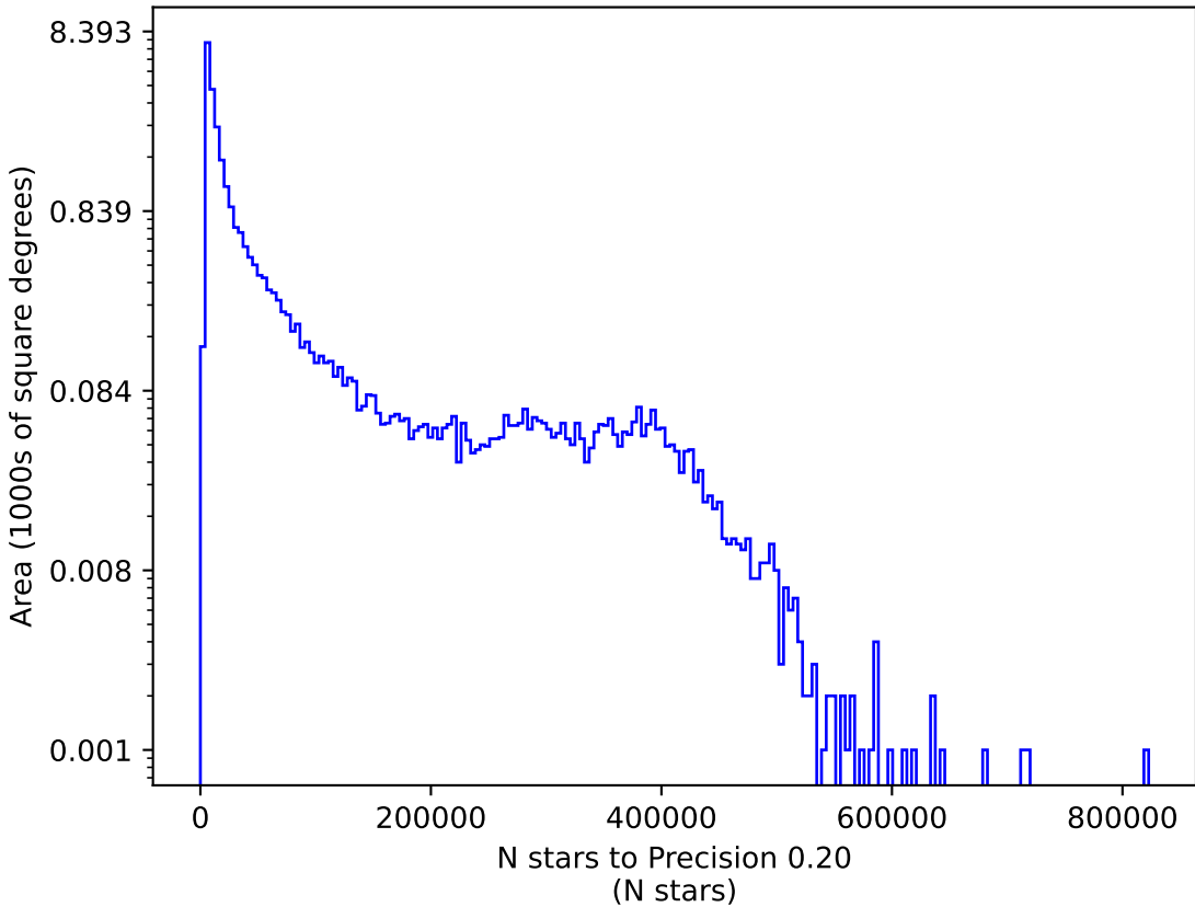
too_elab_r128_d3_ugrizy_v3.4_10yrs g: N stars to Precision 0.20
