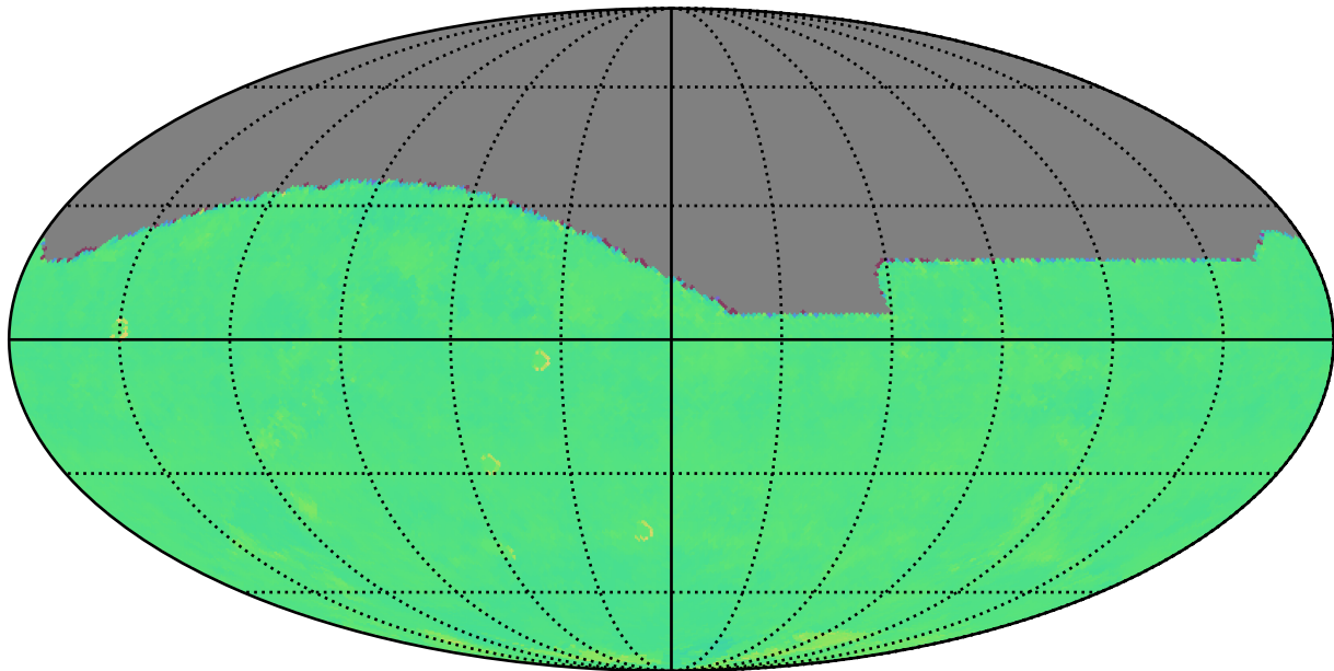
too_elab_r128_d3_ugrizy_v3.4_10yrs r: Kuiper rotTelPos
