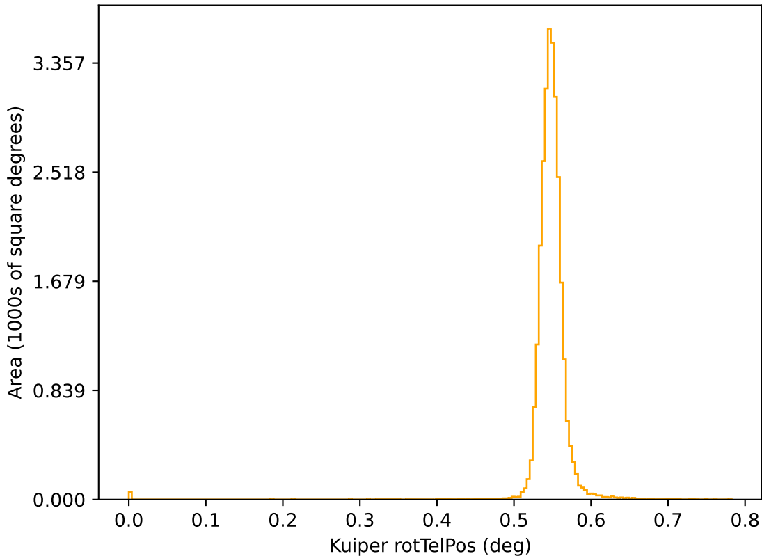
too_elab_r128_d3_ugrizy_v3.4_10yrs r: Kuiper rotTelPos
