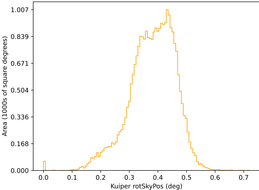
too_elab_r128_d3_ugrizy_v3.4_10yrs r: Kuiper rotSkyPos
