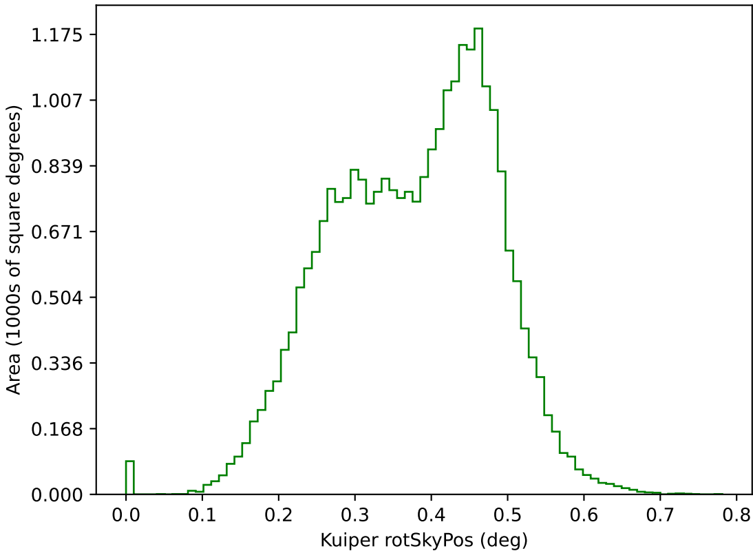
too_elab_r128_d3_ugrizy_v3.4_10yrs g: Kuiper rotSkyPos
