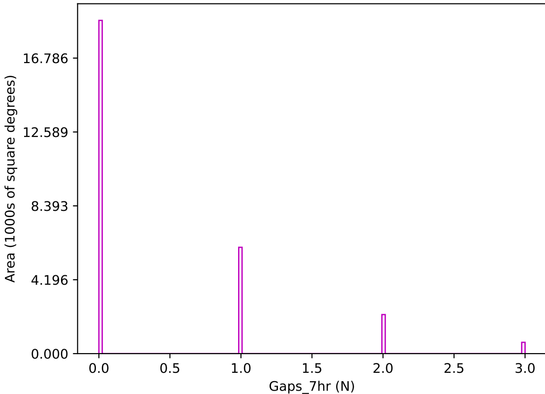
too_elab_r128_d3_ugrizy_v3.4_10yrs z band: Gaps_7hr
