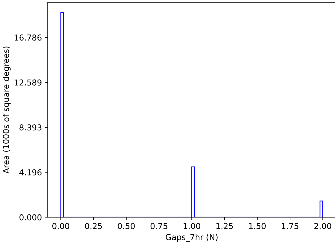
too_elab_r128_d3_ugrizy_v3.4_10yrs y band: Gaps_7hr
