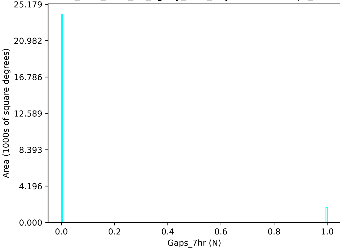
too_elab_r128_d3_ugrizy_v3.4_10yrs u band: Gaps_7hr
