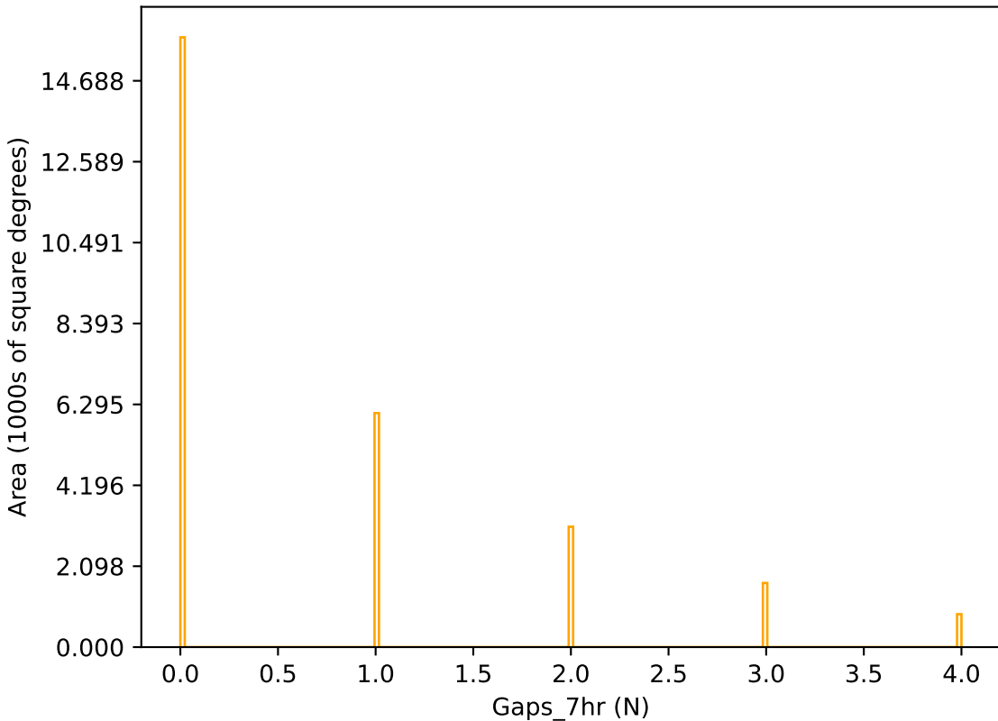
too_elab_r128_d3_ugrizy_v3.4_10yrs r band: Gaps_7hr
