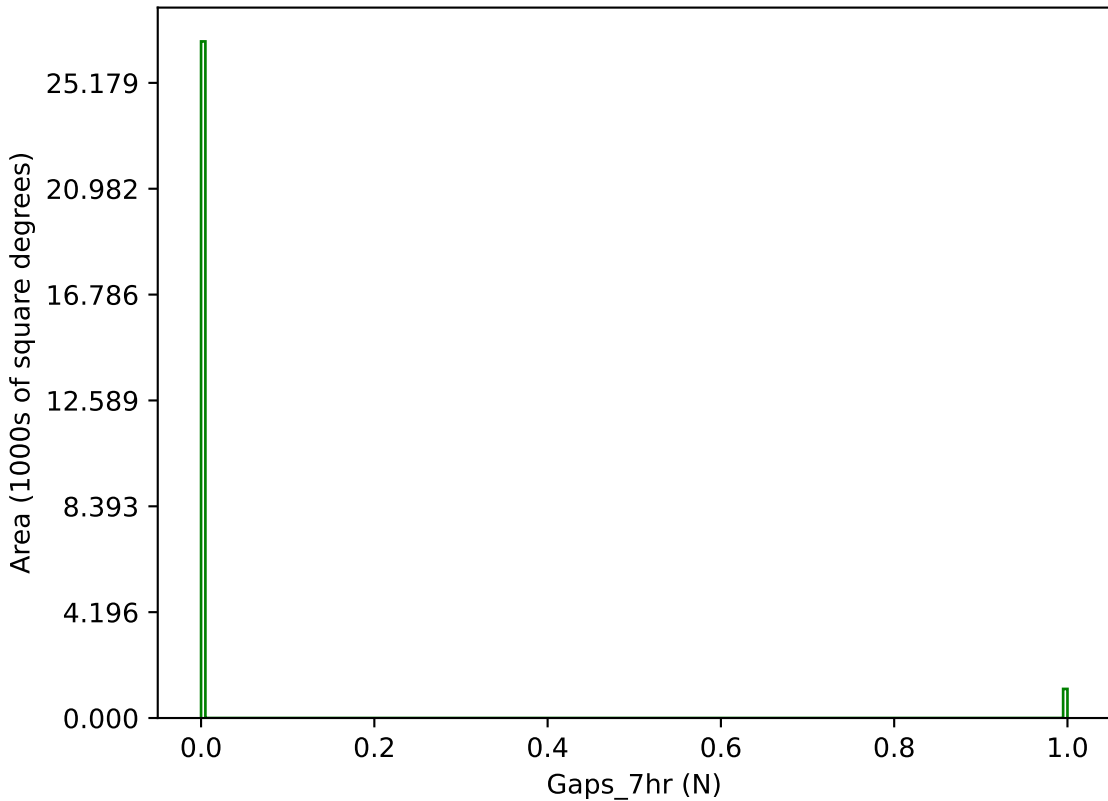
too_elab_r128_d3_ugrizy_v3.4_10yrs g band: Gaps_7hr
