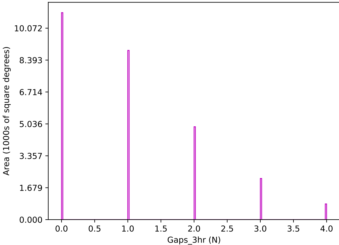
too_elab_r128_d3_ugrizy_v3.4_10yrs z band: Gaps_3hr
