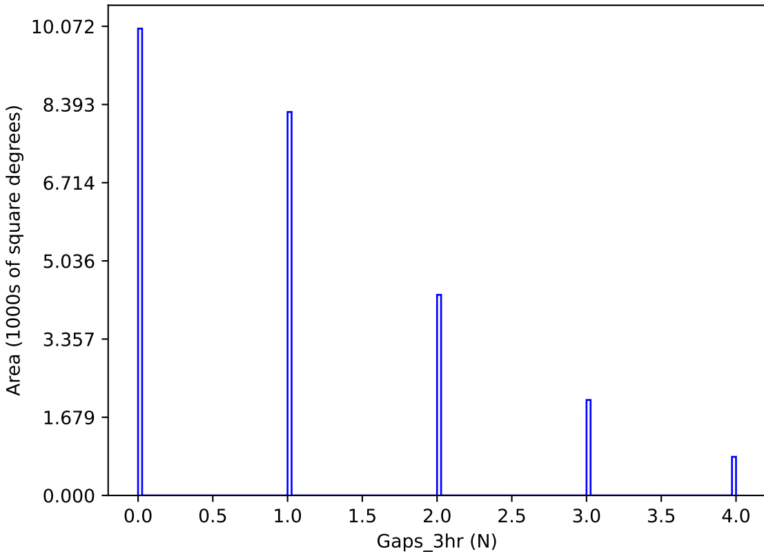
too_elab_r128_d3_ugrizy_v3.4_10yrs y band: Gaps_3hr
