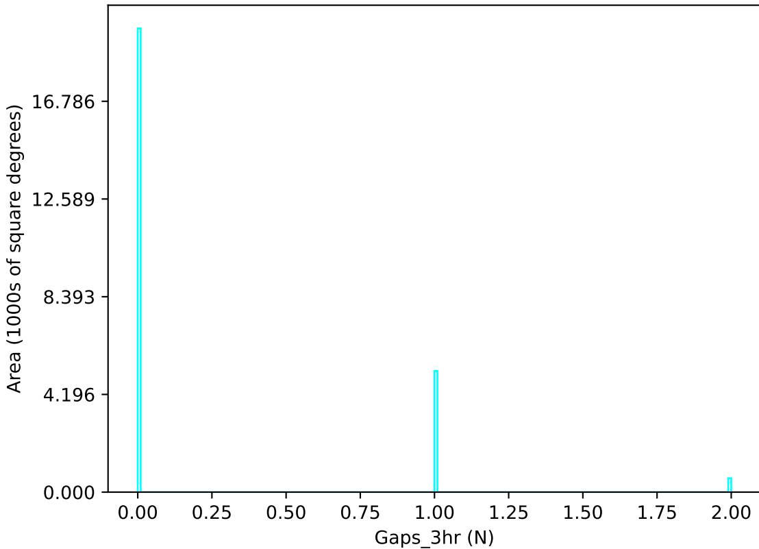
too_elab_r128_d3_ugrizy_v3.4_10yrs u band: Gaps_3hr
