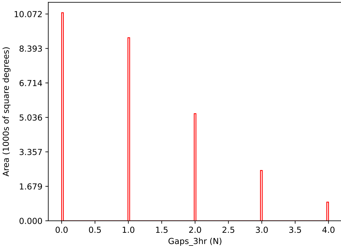
too_elab_r128_d3_ugrizy_v3.4_10yrs i band: Gaps_3hr
