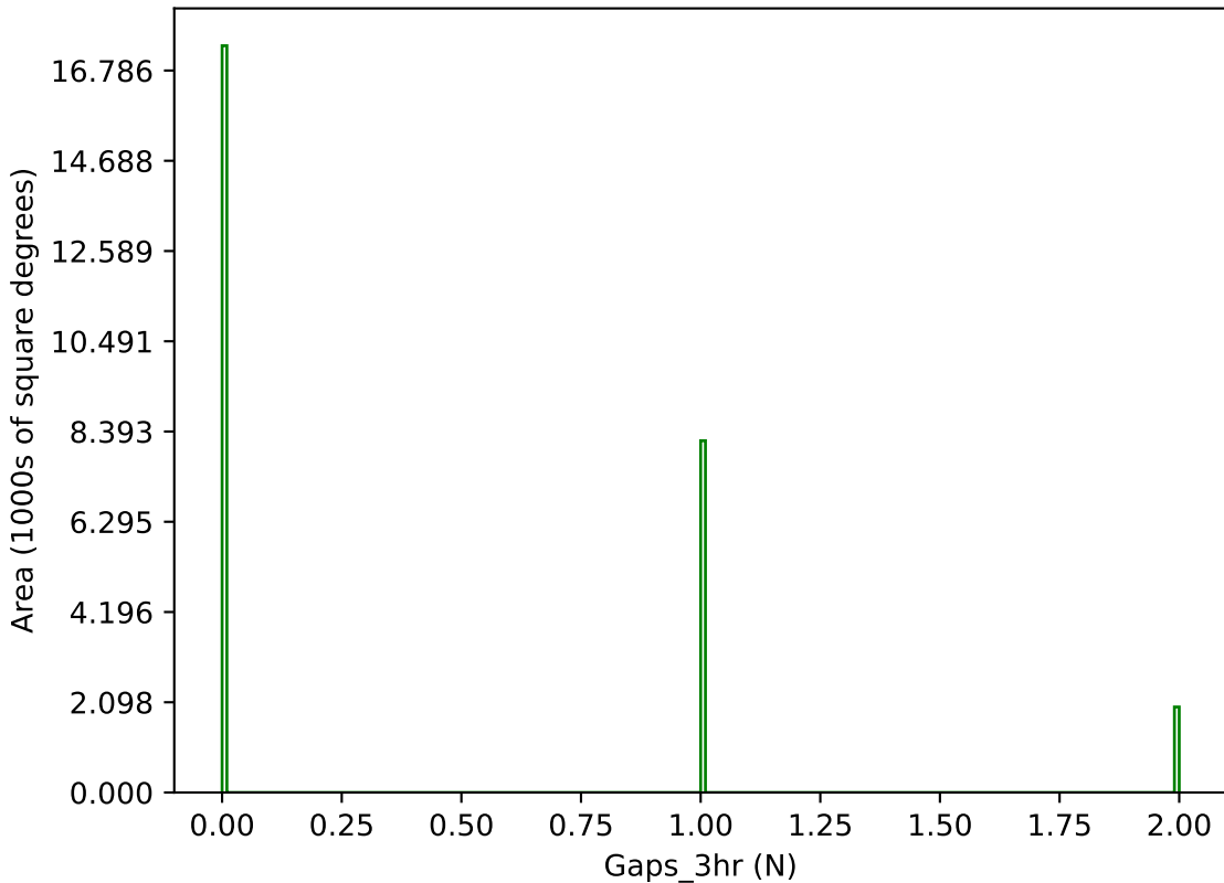
too_elab_r128_d3_ugrizy_v3.4_10yrs g band: Gaps_3hr
