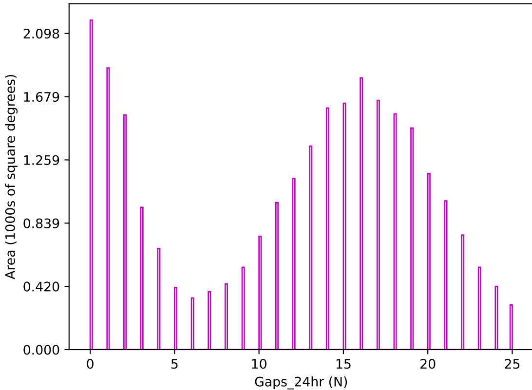
too_elab_r128_d3_ugrizy_v3.4_10yrs z band: Gaps_24hr
