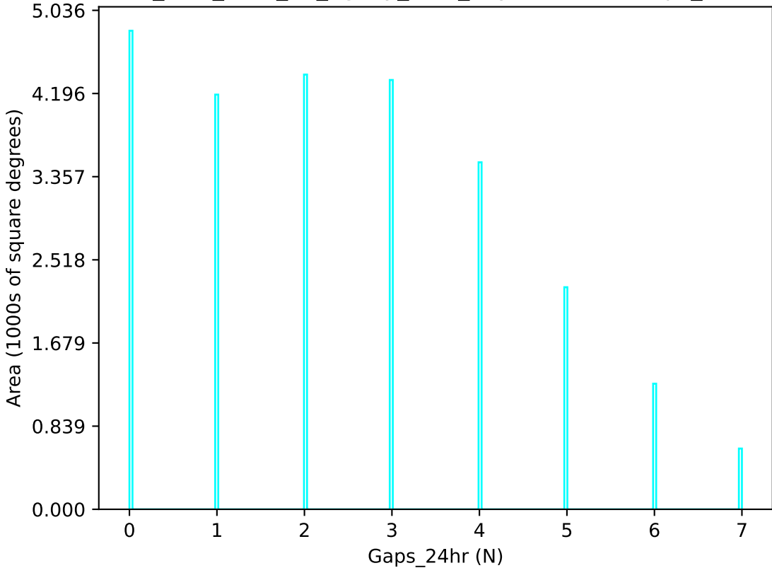
too_elab_r128_d3_ugrizy_v3.4_10yrs u band: Gaps_24hr
