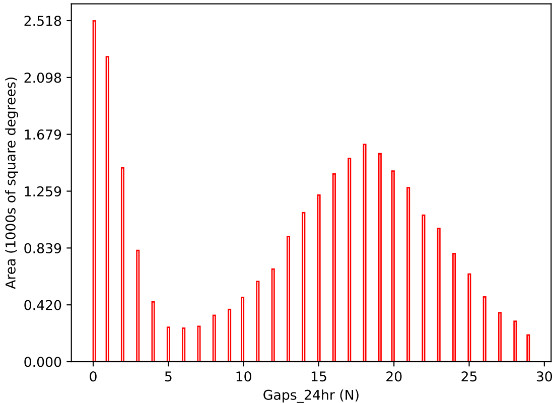
too_elab_r128_d3_ugrizy_v3.4_10yrs i band: Gaps_24hr
