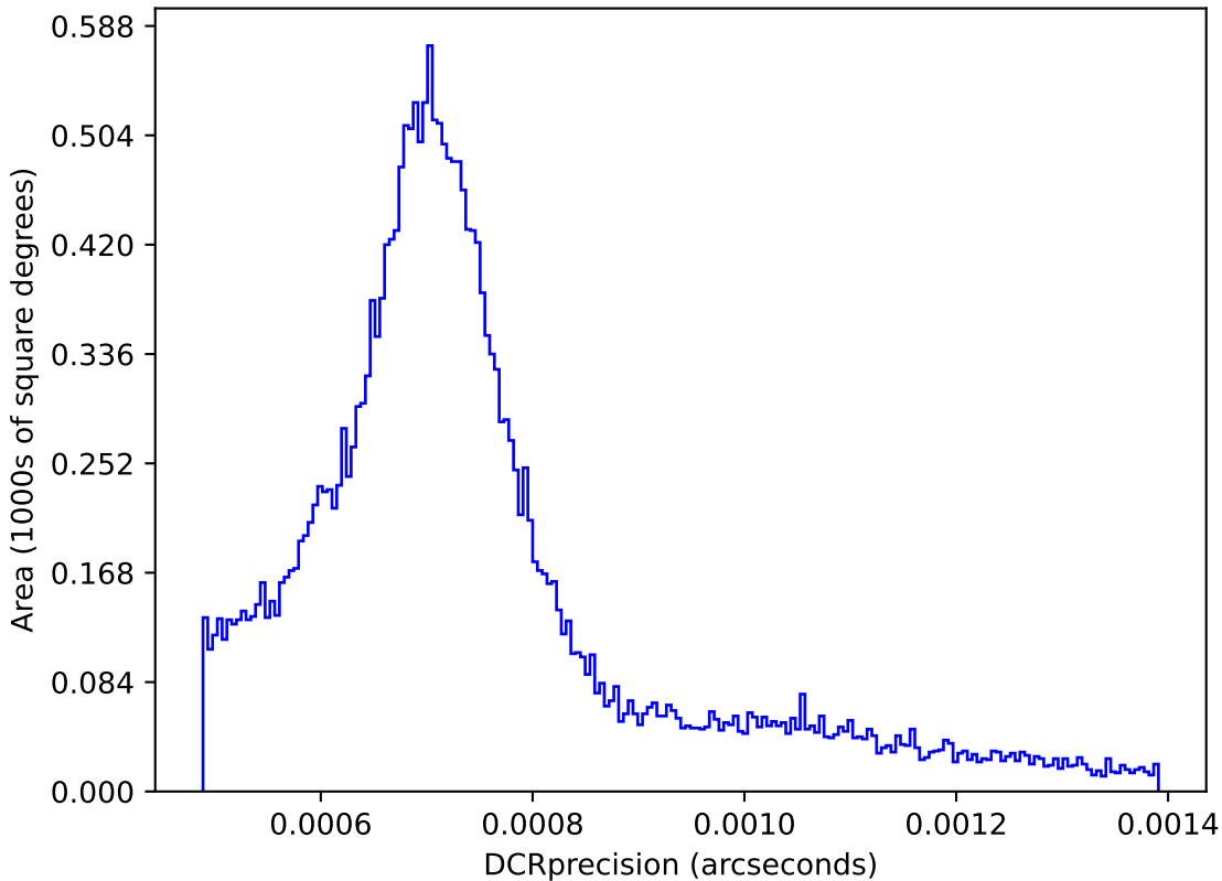
too_elab_r128_d3_ugrizy_v3.4_10yrs : DCRprecision
