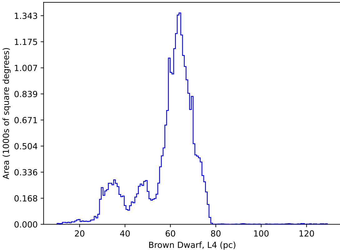
too_elab_r128_d3_ugrizy_v3.4_10yrs : Brown Dwarf, L4
