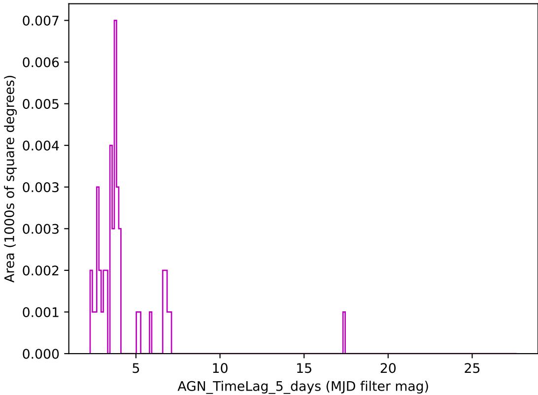
too_elab_r128_d3_ugrizy_v3.4_10yrs z band: AGN_TimeLag_5_days
