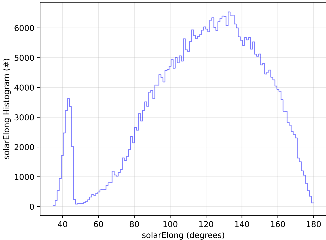
too_elab_r128_d3_ugrizy_v3.4_10yrs WFD z band: solarElong Histogram
