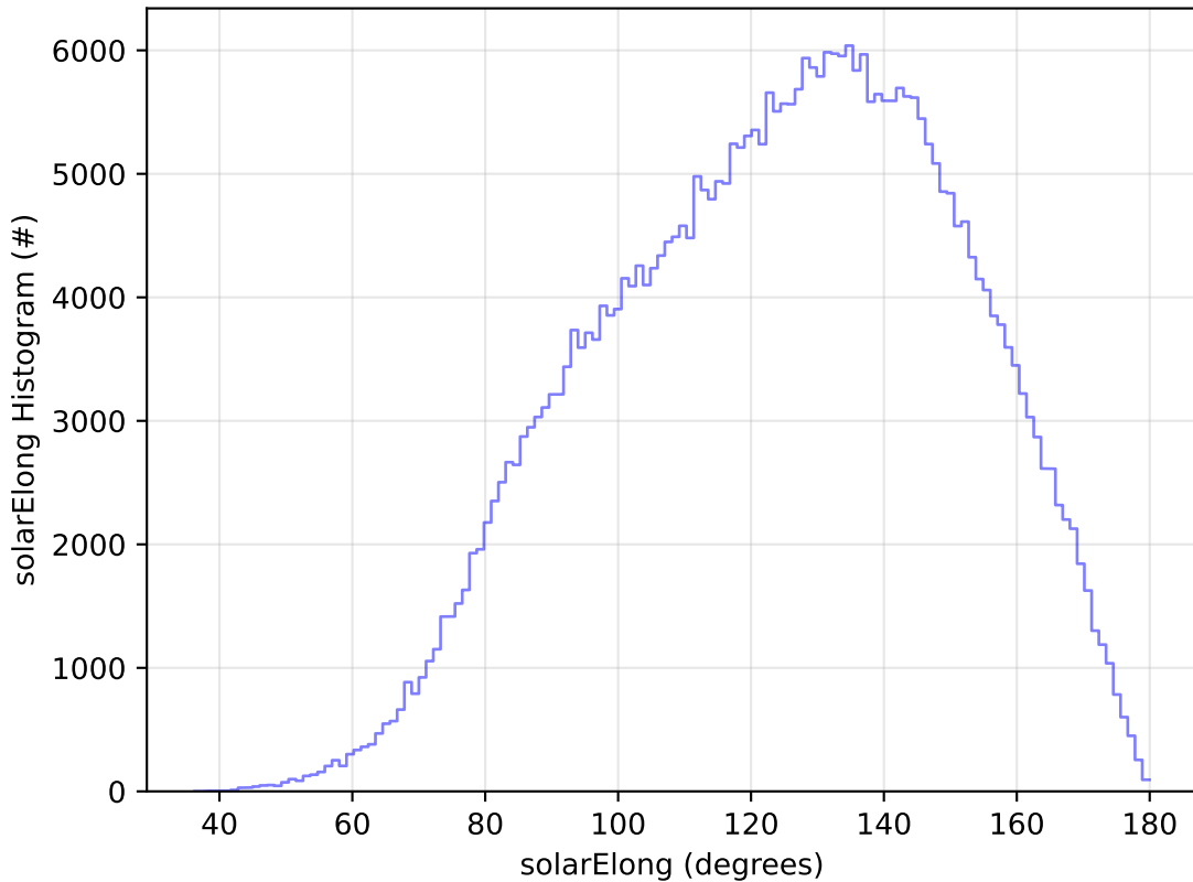
too_elab_r128_d3_ugrizy_v3.4_10yrs WFD y band: solarElong Histogram
