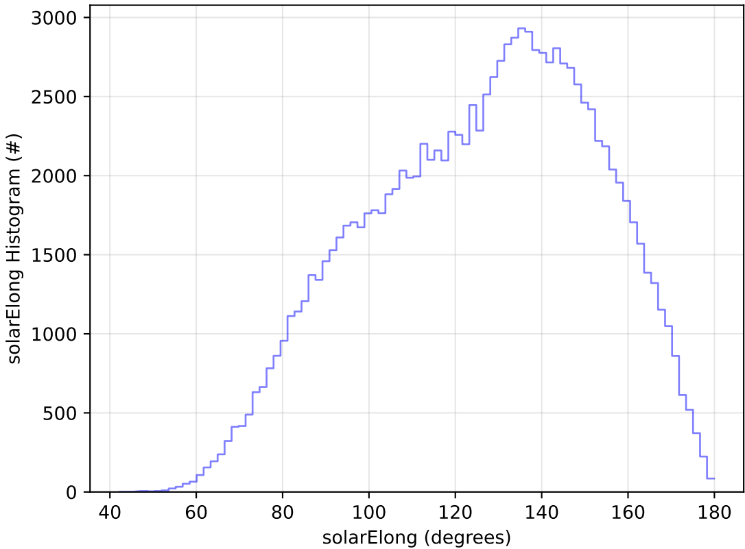
too_elab_r128_d3_ugrizy_v3.4_10yrs WFD u band: solarElong Histogram
