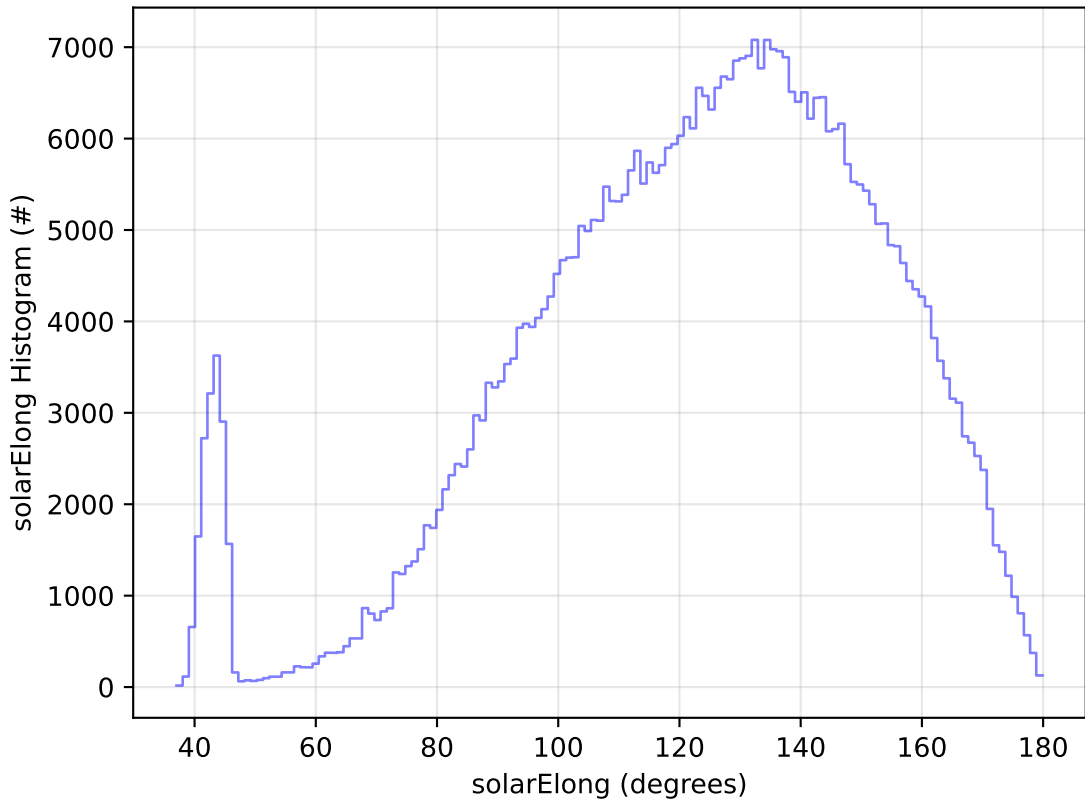
too_elab_r128_d3_ugrizy_v3.4_10yrs WFD r band: solarElong Histogram
