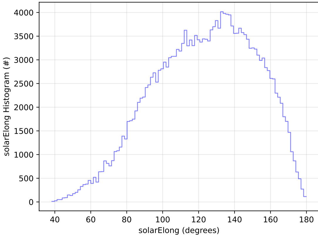
too_elab_r128_d3_ugrizy_v3.4_10yrs WFD g band: solarElong Histogram
