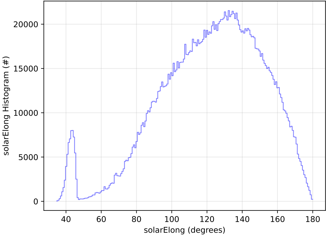
too_elab_r128_d3_ugrizy_v3.4_10yrs WFD all bands: solarElong Histogram
