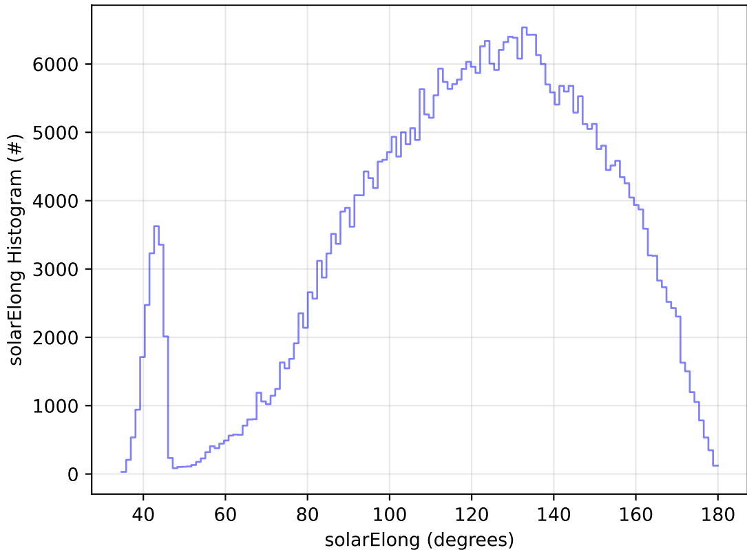
too_elab_r128_d3_ugrizy_v3.4_10yrs All sky z band: solarElong Histogram
