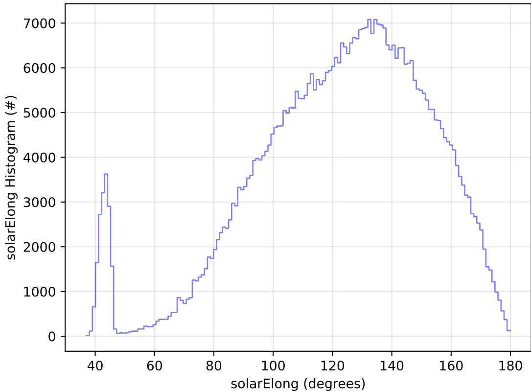
too_elab_r128_d3_ugrizy_v3.4_10yrs All sky r band: solarElong Histogram
