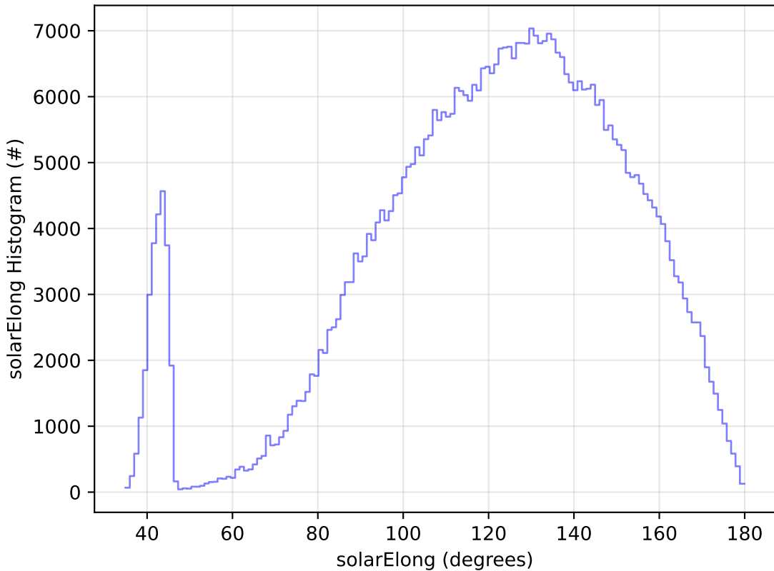
too_elab_r128_d3_ugrizy_v3.4_10yrs All sky i band: solarElong Histogram
