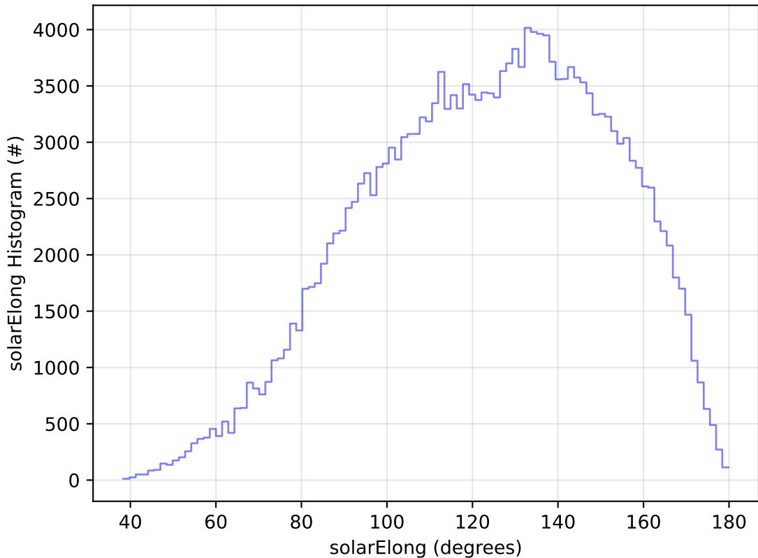
too_elab_r128_d3_ugrizy_v3.4_10yrs All sky g band: solarElong Histogram
