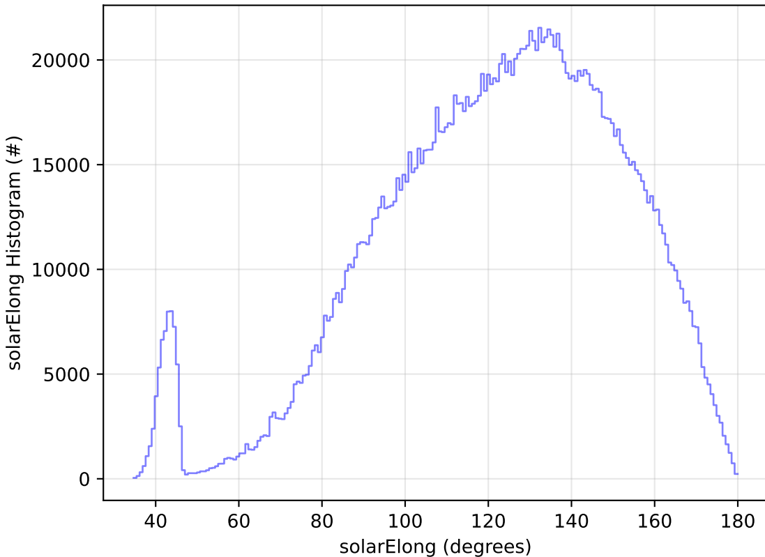
too_elab_r128_d3_ugrizy_v3.4_10yrs All sky all bands: solarElong Histogram
