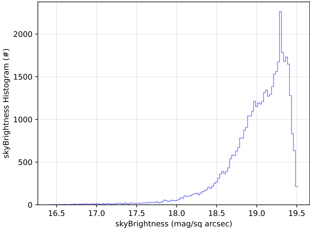
too_elab_r128_d3_ugrizy_v3.4_10yrs Yr 1 z band: skyBrightness Histogram
