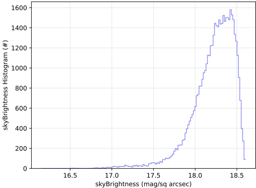
too_elab_r128_d3_ugrizy_v3.4_10yrs Yr 1 y band: skyBrightness Histogram
