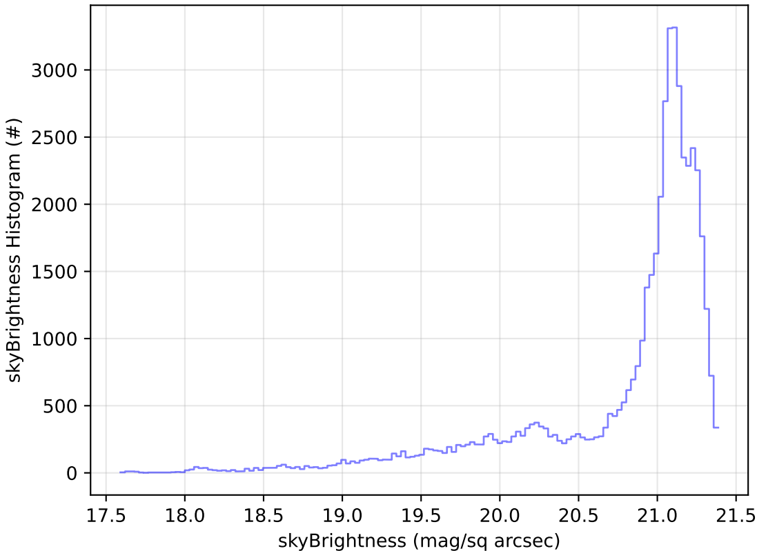
too_elab_r128_d3_ugrizy_v3.4_10yrs Yr 1 r band: skyBrightness Histogram
