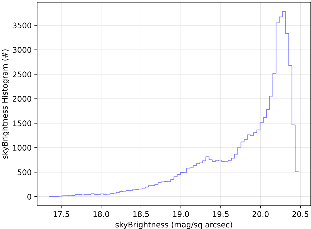
too_elab_r128_d3_ugrizy_v3.4_10yrs Yr 1 i band: skyBrightness Histogram
