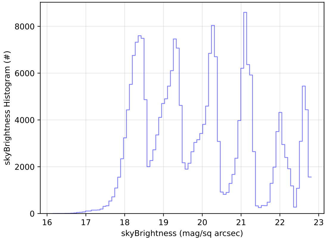
too_elab_r128_d3_ugrizy_v3.4_10yrs Yr 1 all bands: skyBrightness Histogram
