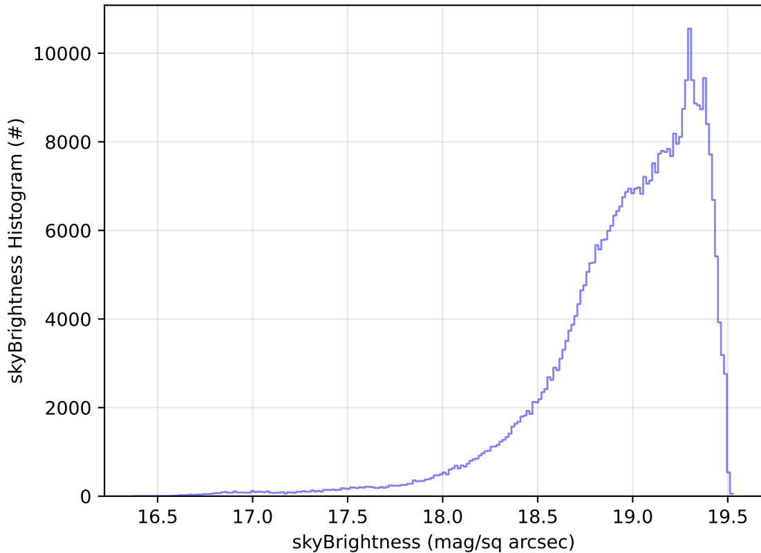
too_elab_r128_d3_ugrizy_v3.4_10yrs WFD z band: skyBrightness Histogram
