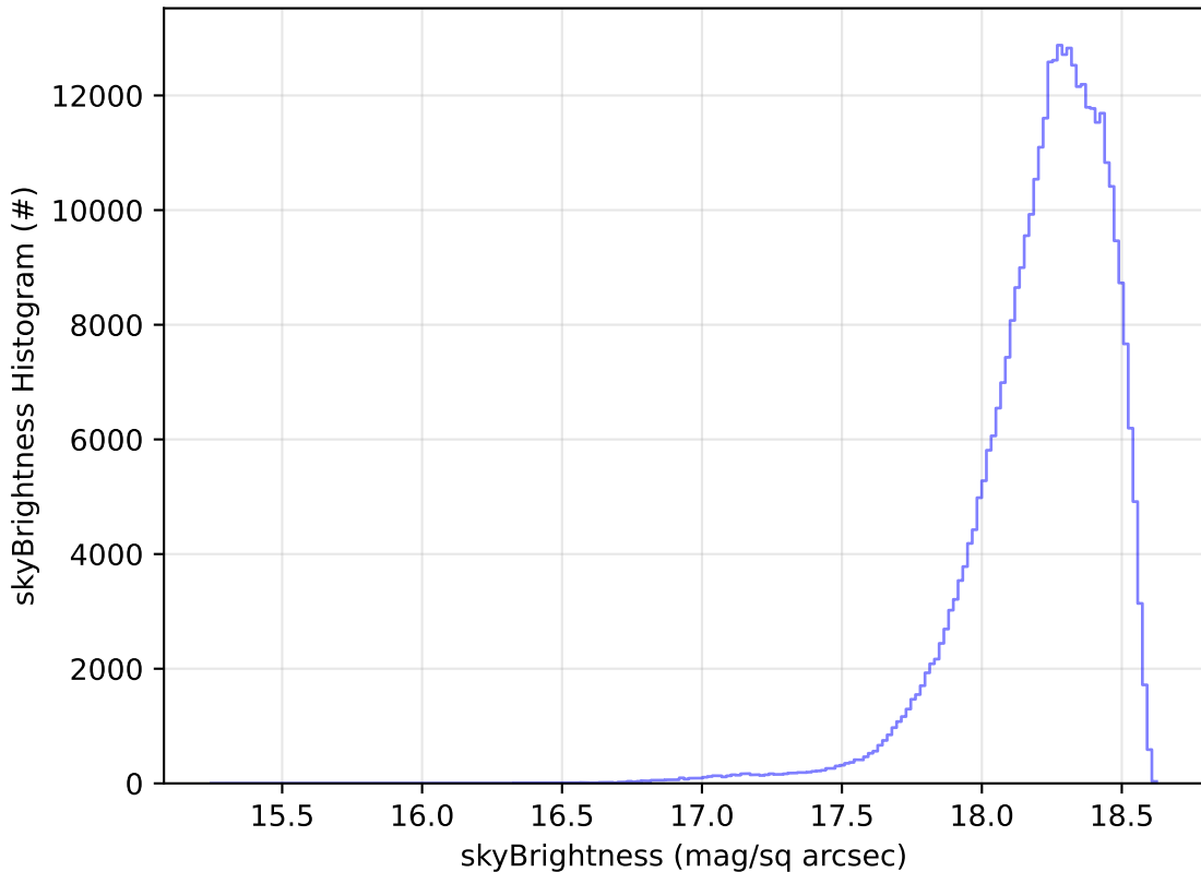
too_elab_r128_d3_ugrizy_v3.4_10yrs WFD y band: skyBrightness Histogram
