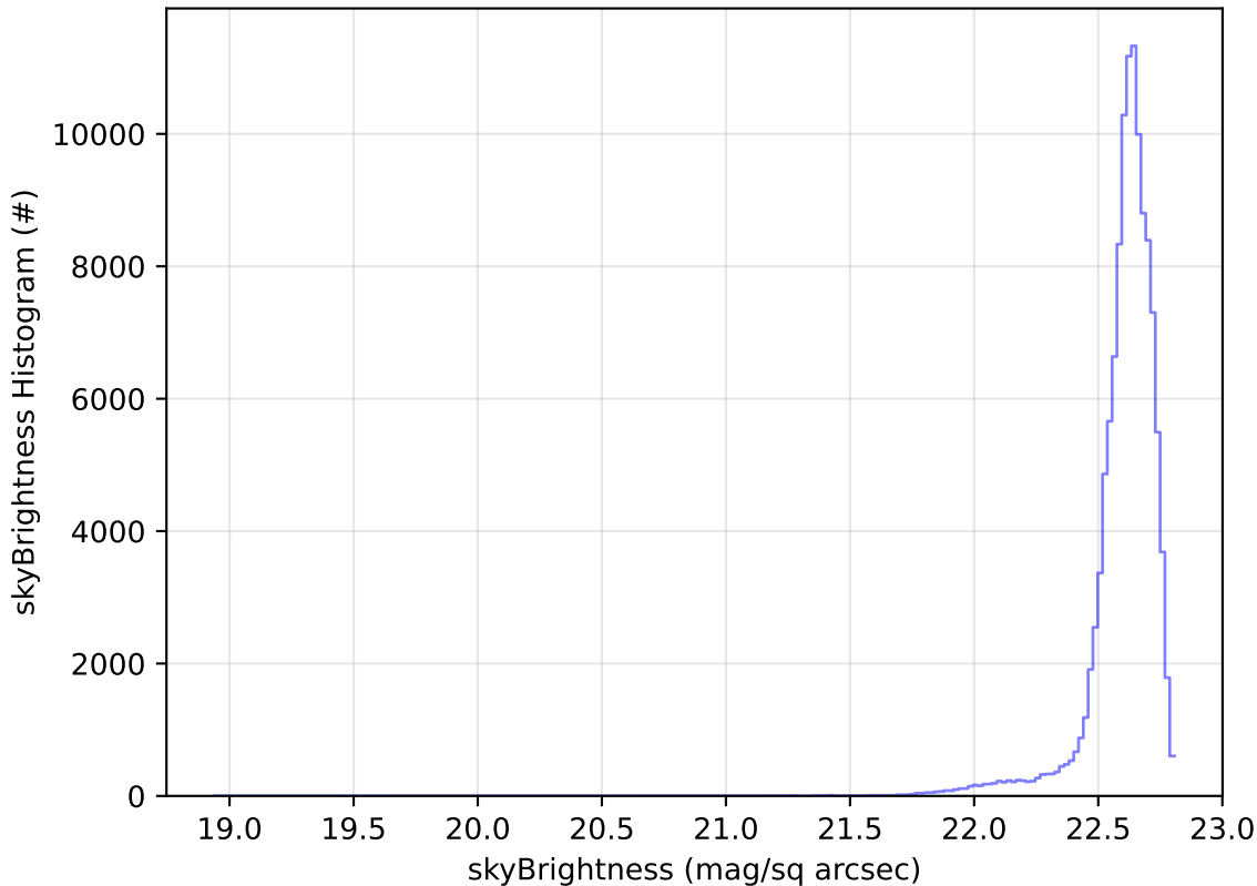
too_elab_r128_d3_ugrizy_v3.4_10yrs WFD u band: skyBrightness Histogram
