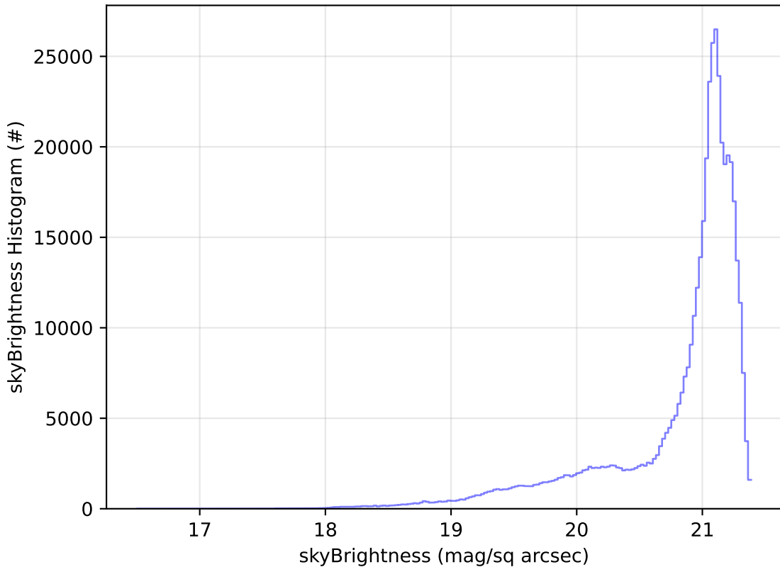
too_elab_r128_d3_ugrizy_v3.4_10yrs WFD r band: skyBrightness Histogram
